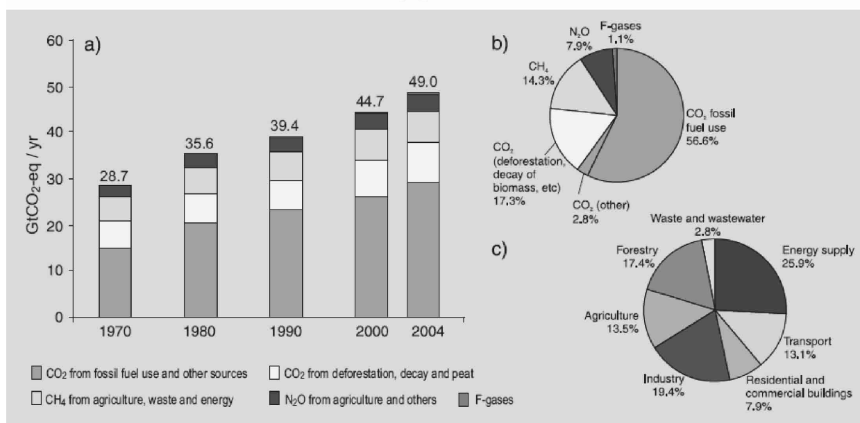
Global anthropogenic GHG emissions
